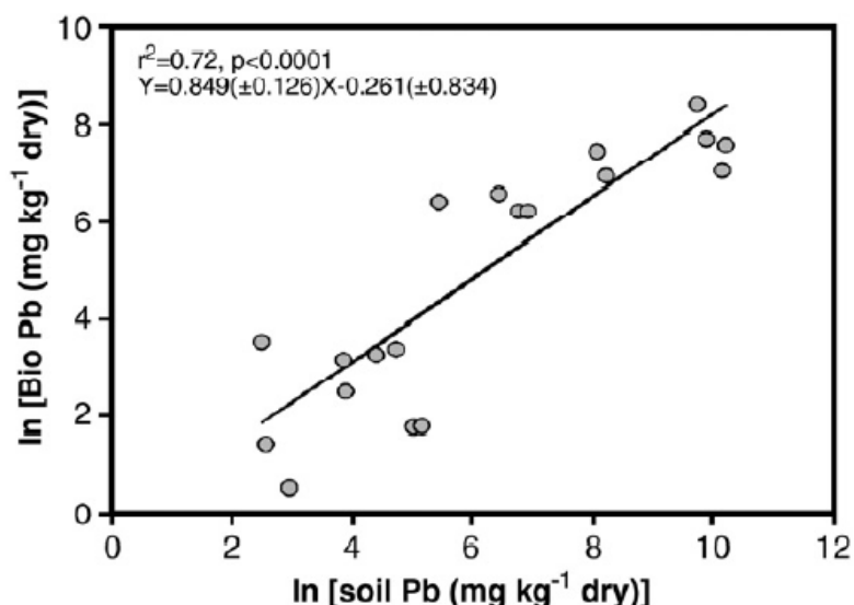
Figure 1-20 Correlation between ln-transformed bioaccessible lead concentrations in vegetation and soil lead concentrations (Bennett et al., 2007)
