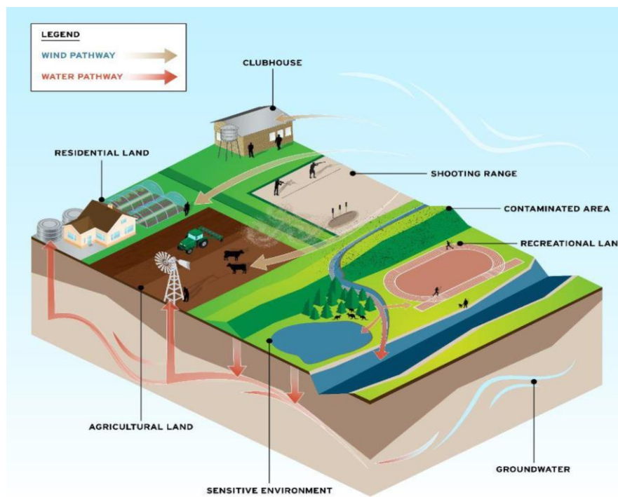
Figure 1-19 Simplified model of water and wind pathways that can spread lead off site from a shooting range (Australian EPA, 2019) Note: indicative only and not to scale.
