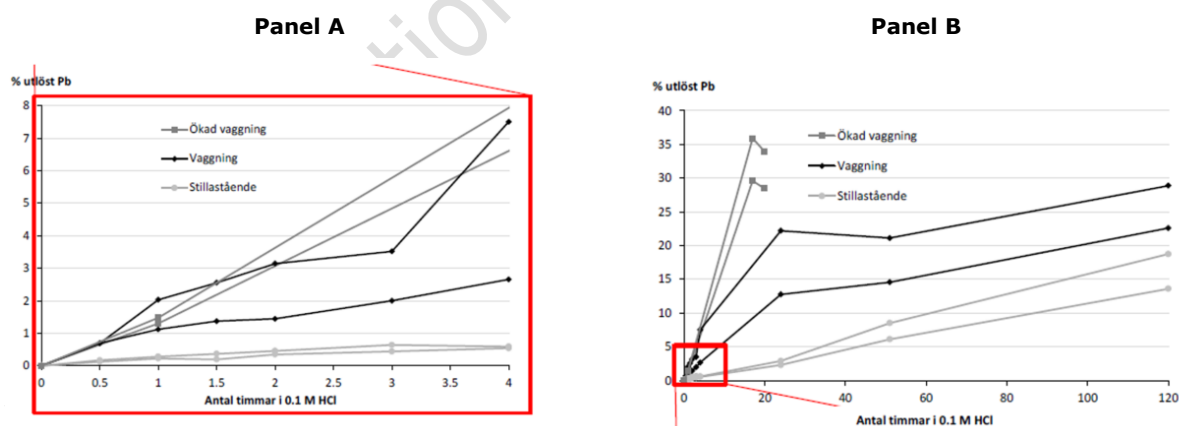
Figure 1-21: Percentage of lead released in stomach-like environment (0.1 M hydrochloric acid) after a certain time with heavy rocking (Ökad vagging), rocking (Vagging) or without rocking (Stillastående) (Forsell et al., 2014).
