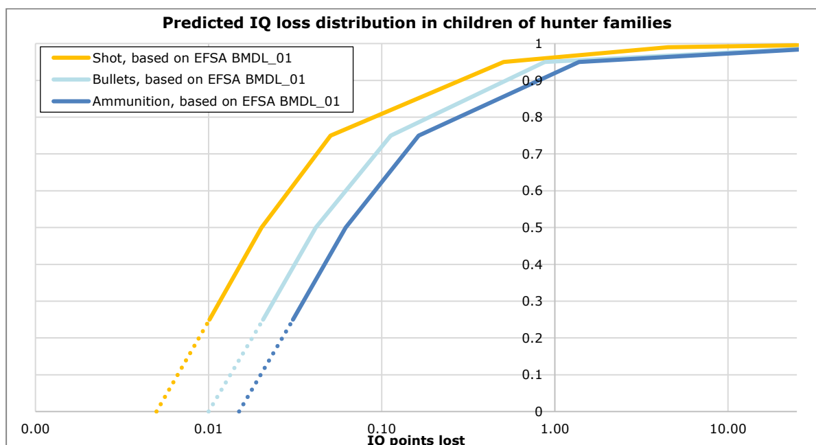
Figure 2-2: Empirical cumulative distribution functions (ECDFs) of IQ loss in high-frequency game meat consumers.
