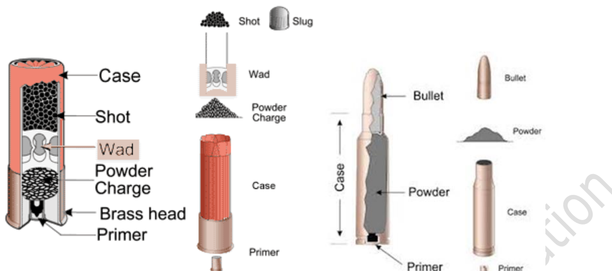
Figure 1-1: Examples of gunshot (left hand-side) and other types of projectiles (e.g. bullet on the right hand-side) within the scope of the proposed restriction
