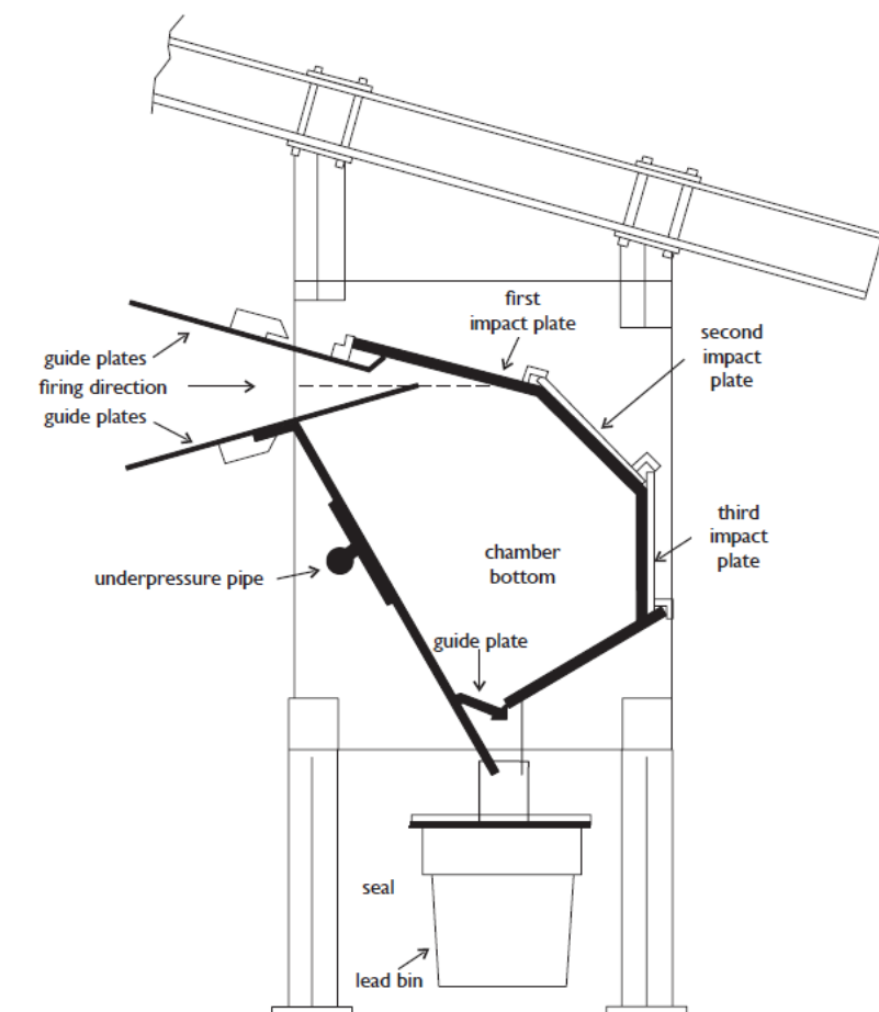
Figure 1-8 Example of a total containment bullet trap (Kajander and Parri, 2014)
