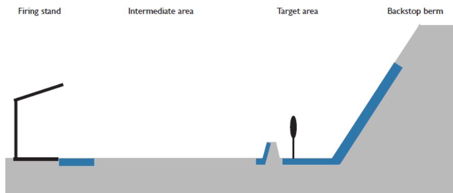
Figure 1-11 Contamination hotspot areas at a rifle or pistol range (Kajander and Parri, 2014)
