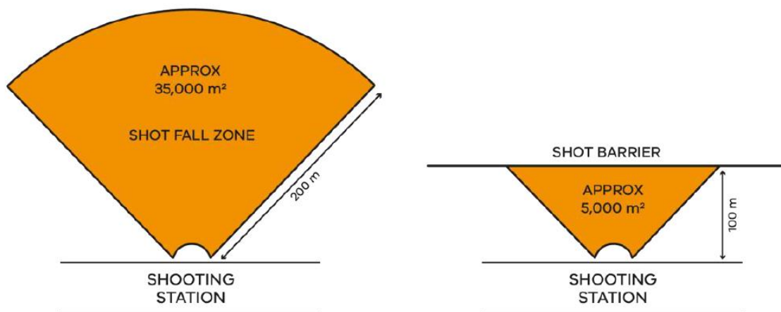
Figure 1-4 Reduction in the shot fall zone by using a barrier at a trap station (Australian EPA, 2019)
