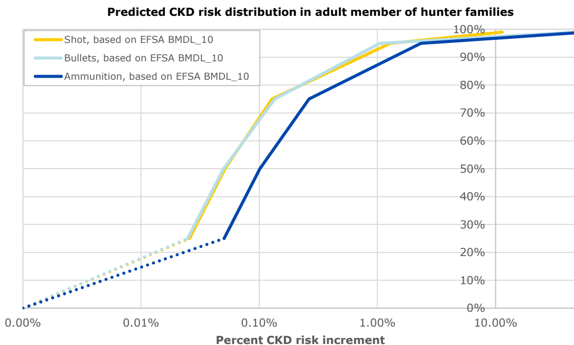
Figure 2-3: Empirical cumulative distribution functions (ECDFs) of excess CKD risk in adult high-frequency game meat consumers.
